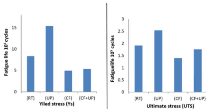
Figure 9: Fatigue life testing of different conditions based on mechanical properties.
